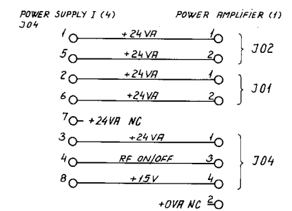
CABLE 7 : POWER SUPPLY I TO POWER AMPLIFIER
