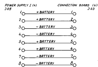
CABLE 4 : POWER SUPPLY I TO CONNECTION BOARD
