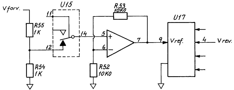
Figure 6: Measuring RHO
